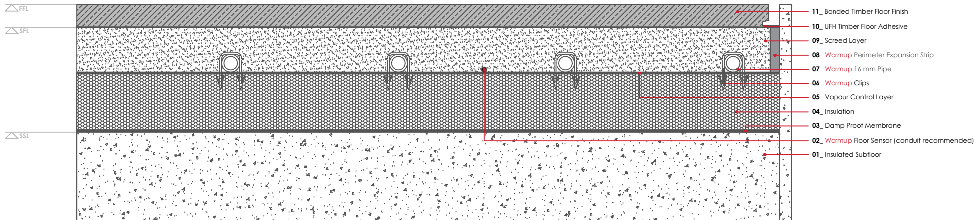
WARMUP CLYPSO Bonded timber floor finish
