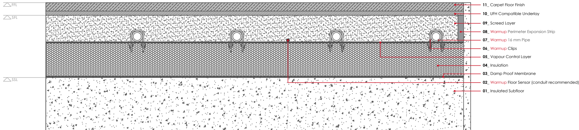
WARMUP CLYPSO SYSTEM. Carpet floor finish
