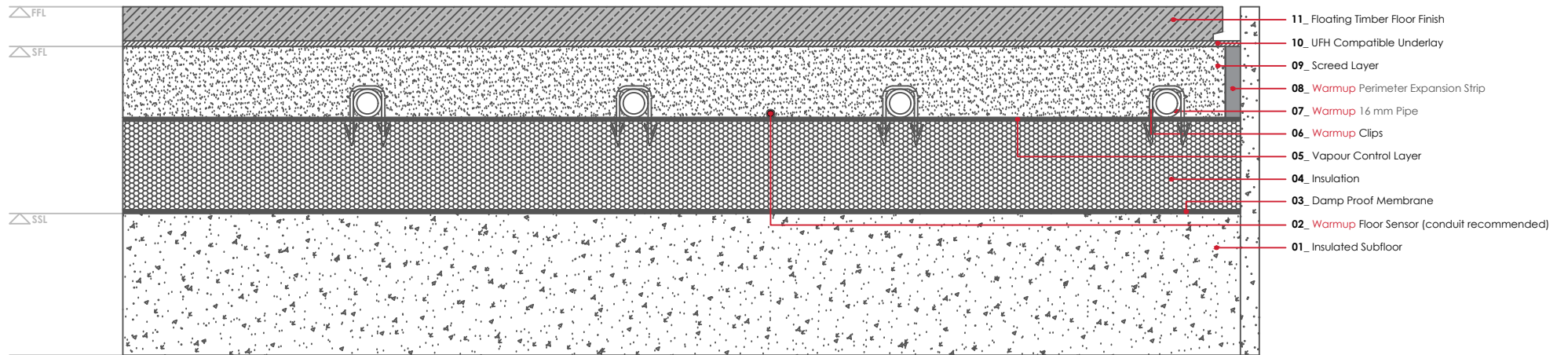
WARMUP CLYPSO Floating timber floor finish
