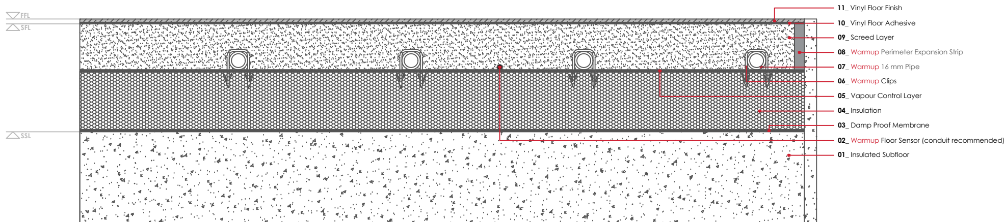
WARMUP CLYPSO SYSTEM. Vinyl floor finish - glued
