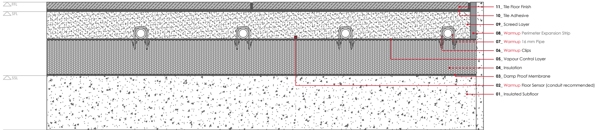
WARMUP CLYPSO SYSTEM. Tiled floor finish
