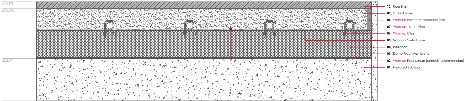
WARMUP CLYPSO SYSTEM. Standard Detail
