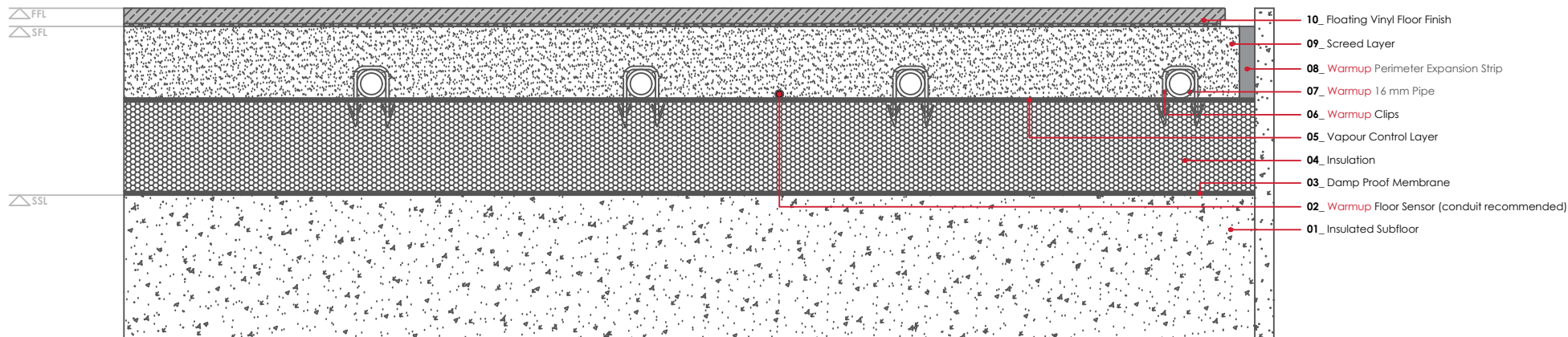
WARMUP CLYPSO SYSTEM. Vinyl floor finish - floating
