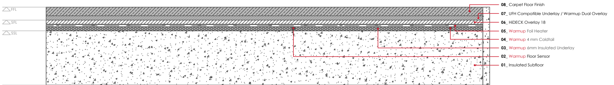
WARMUP FOIL HEATER SYSTEM. Carpet floor finish
