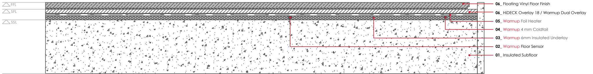
WARMUP FOIL HEATER SYSTEM. Vinyl floor finish - floating
