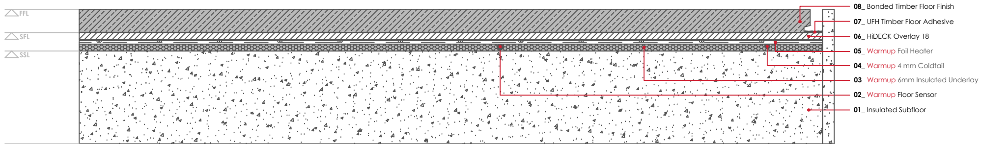
WARMUP FOIL HEATER SYSTEM Bonded timber floor finish
