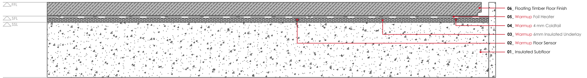
WARMUP FOIL HEATER SYSTEM Floating timber floor finish
