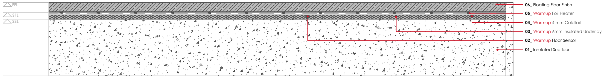
WARMUP FOIL HEATER SYSTEM. Standard Detail
