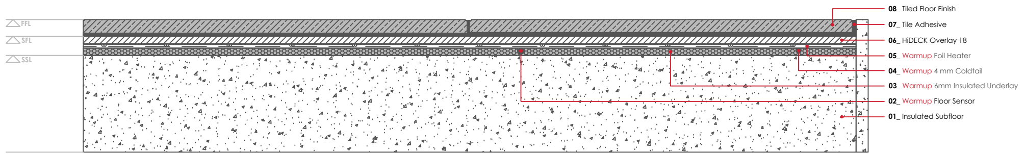
WARMUP FOIL HEATER SYSTEM Tiled floor finish
