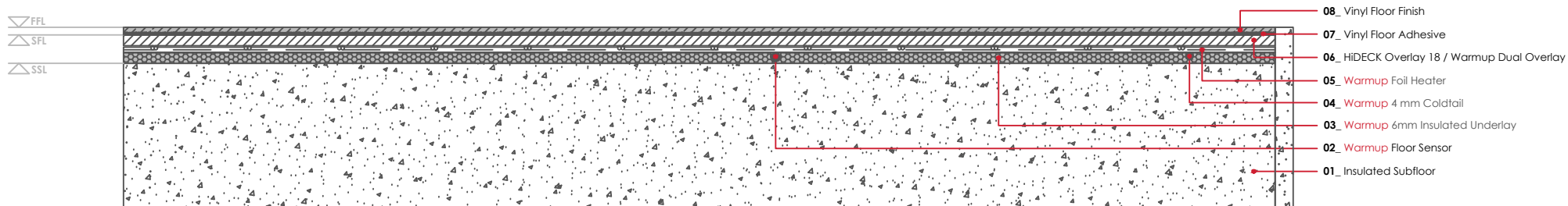
WARMUP FOIL HEATER SYSTEM. Vinyl floor finish - glued
