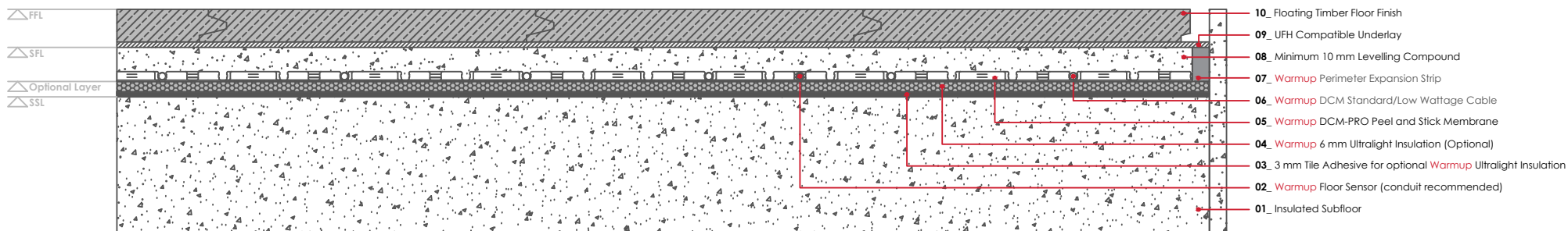
WARMUP DCM-PRO SYSTEM. Floating timber floor finish
