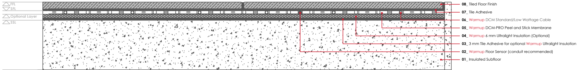
WARMUP DCM-PRO SYSTEM. Tiled floor finish
