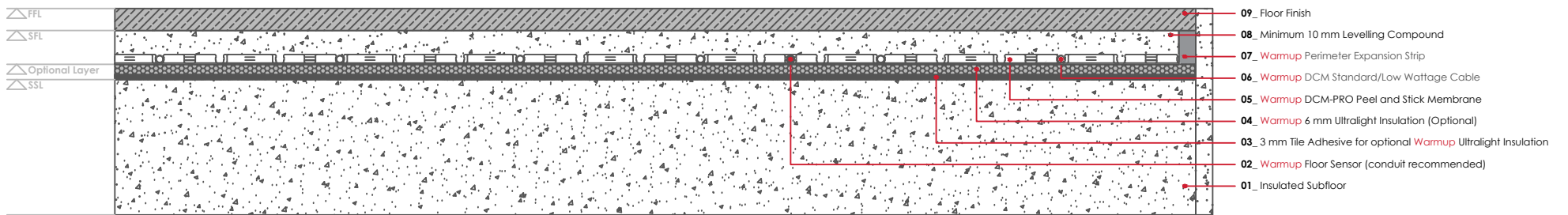
WARMUP DCM-PRO SYSTEM. Standard Detail
