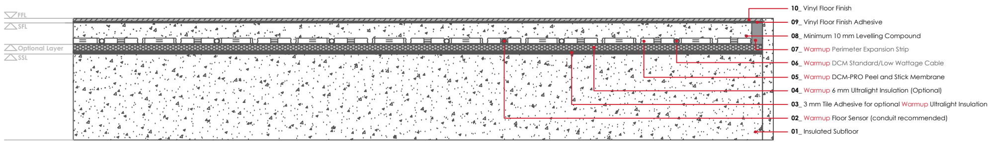
WARMUP DCM-PRO SYSTEM. Vinyl floor finish - glued
