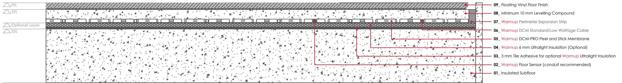
WARMUP DCM-PRO SYSTEM. Floating vinyl floor finish
