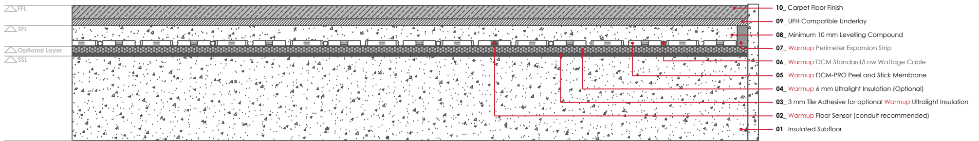
WARMUP DCM-PRO SYSTEM. Carpet floor finish
