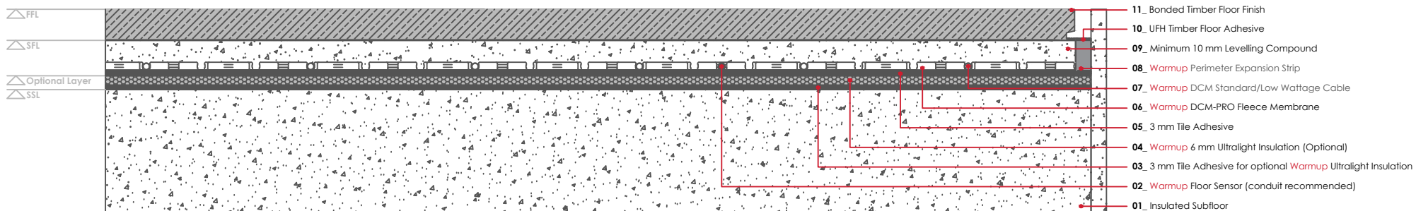
WARMUP DCM-PRO SYSTEM. Bonded timber floor finish
