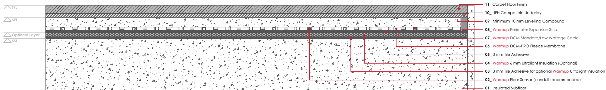
WARMUP DCM-PRO SYSTEM. Carpet floor finish
