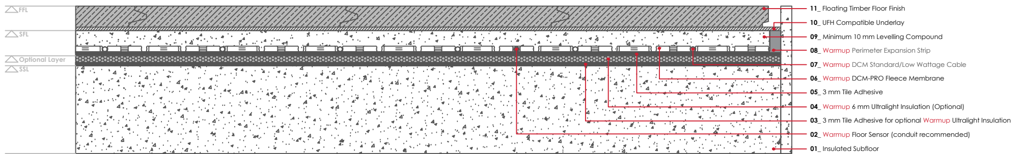
WARMUP DCM-PRO SYSTEM. Floating timber floor finish
