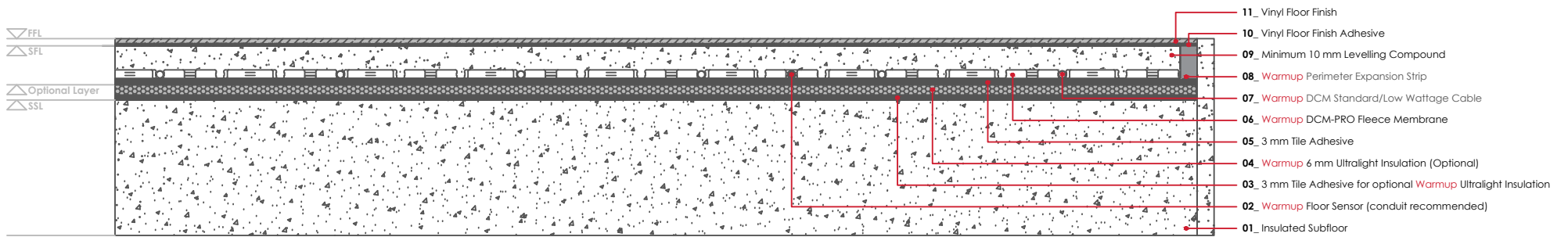
WARMUP DCM-PRO SYSTEM. Vinyl floor finish - glued
