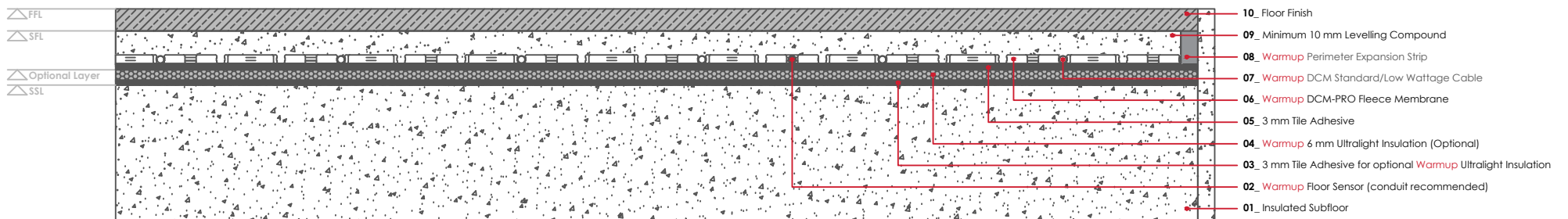
WARMUP DCM-PRO SYSTEM. Standard Detail
